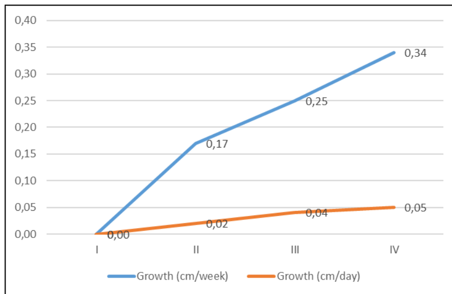
Figure 6. Coral growth rate using the spider module.
