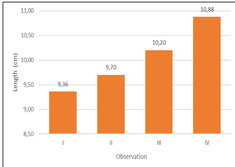
Figure 3. Coral growth using spider modules
